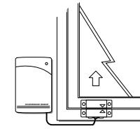
Sliding window
